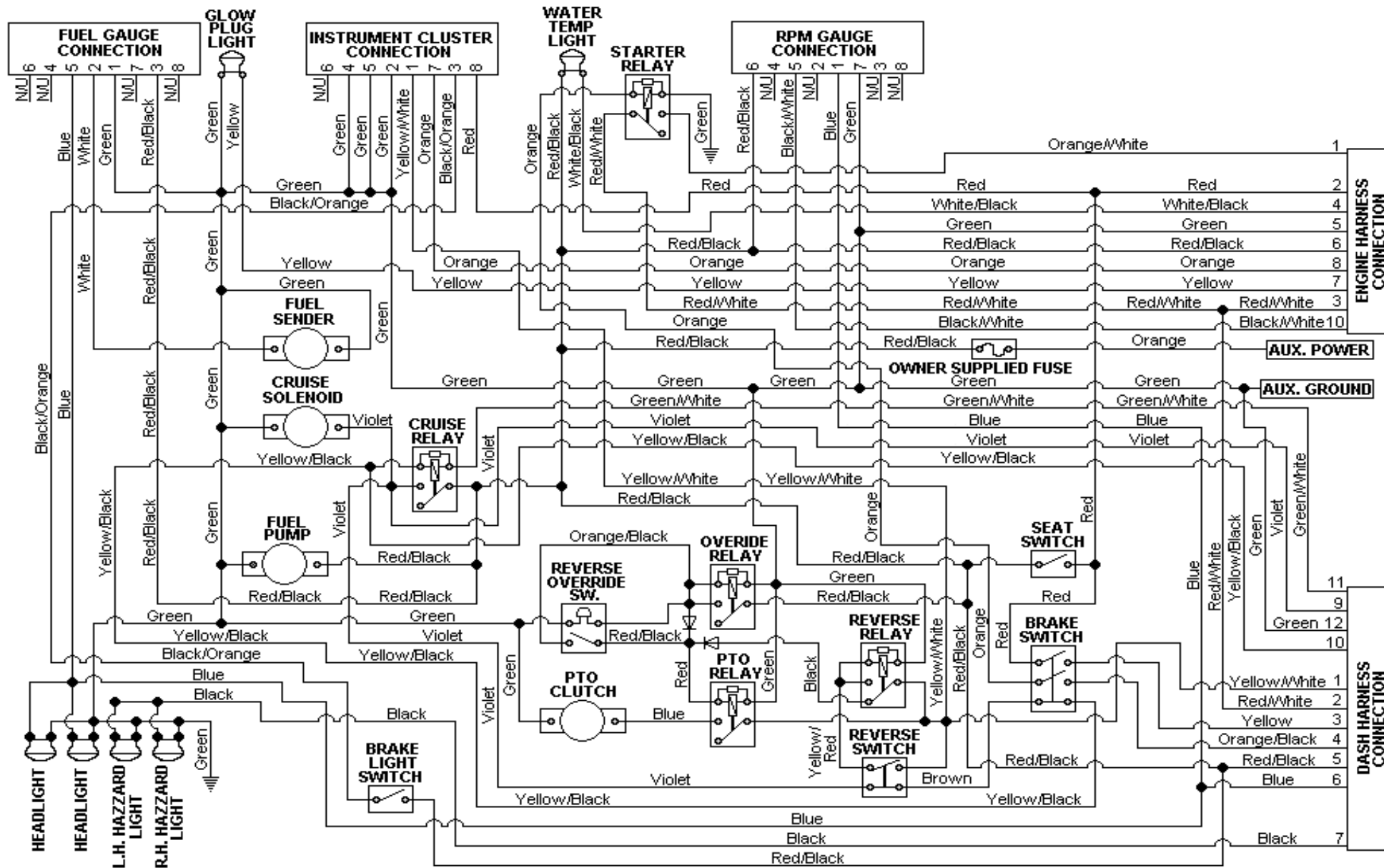
MODEL 5264D MAIN HARNESS (2006) HARNESS NUMBER (629-04128)
