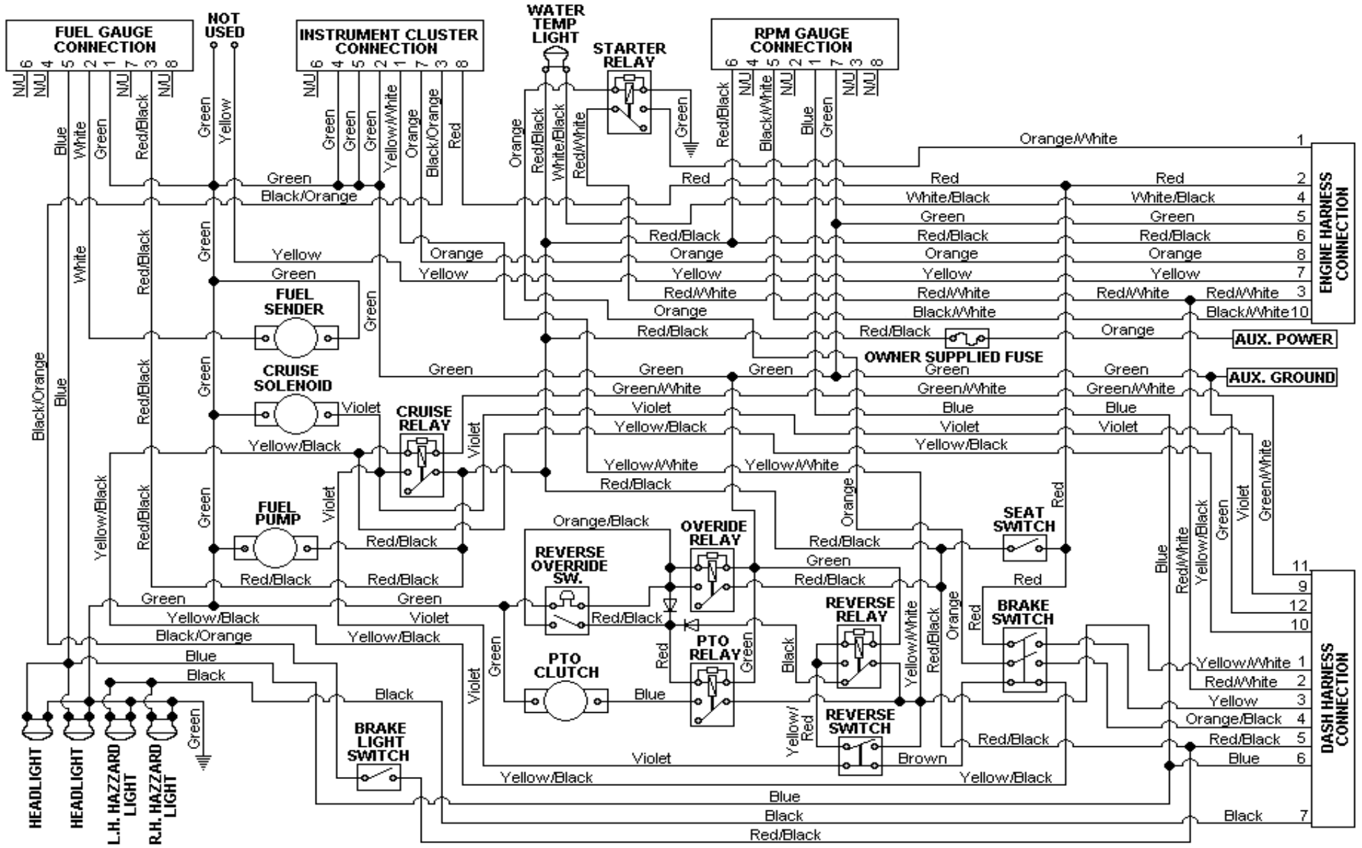
MODEL 5254 MAIN HARNESS (05-06) HARNESS NUMBER (629-04128)
